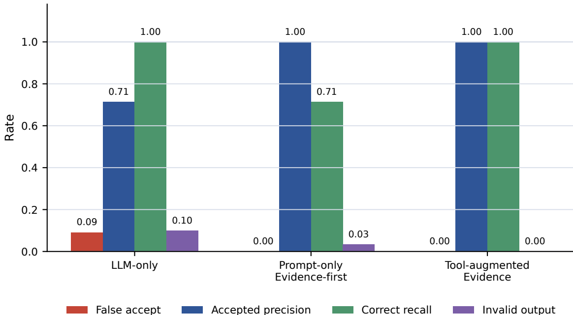
Safety/recall tradeoff across review conditions
