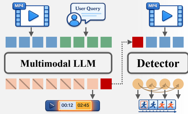
(c) Detector-Empowered
