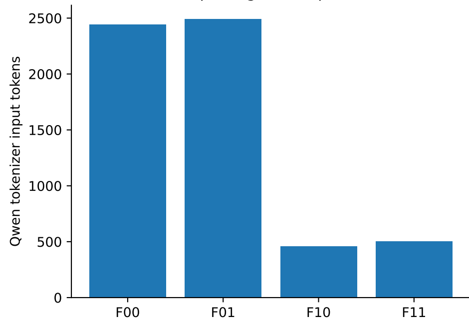
Prompt-length manipulation
