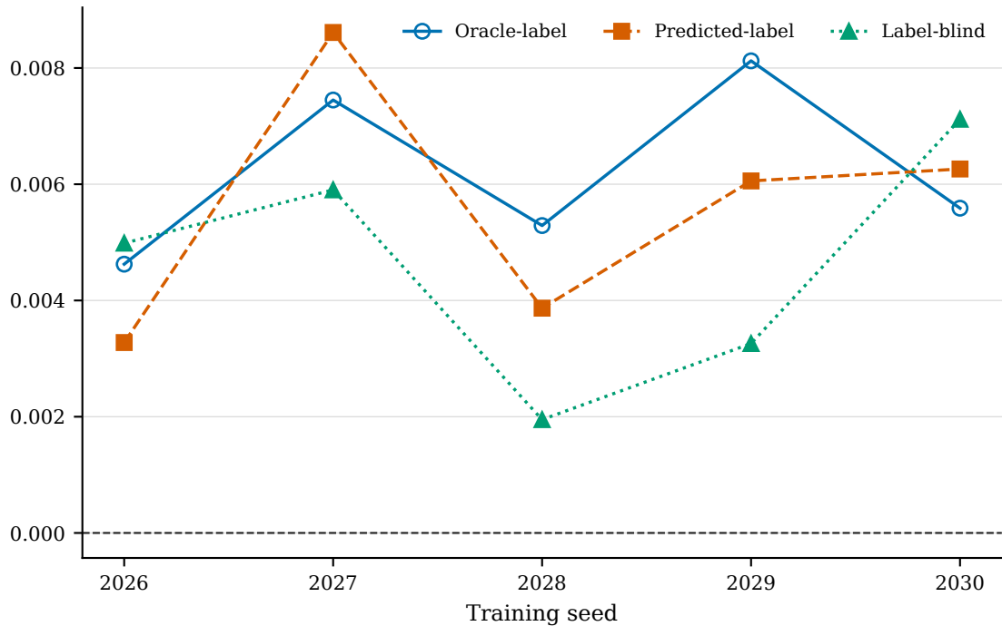
K=3 F1 difference from BM25
