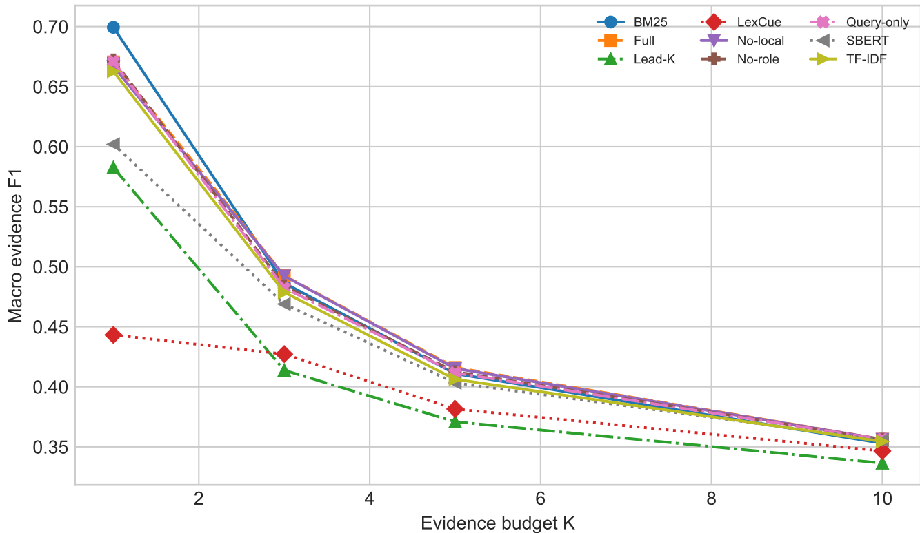
Finite extraction family: oracle
