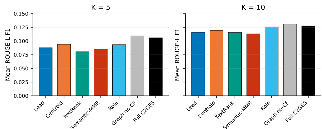
Figure 3. Mean Executive-Summary ROUGE-L F1 for the seven frozen conditions ( n = 15 reports). Bars are descriptive macro-means; paired distributions and sensitivity results appear in Figure 4 and Tables 4–5.
