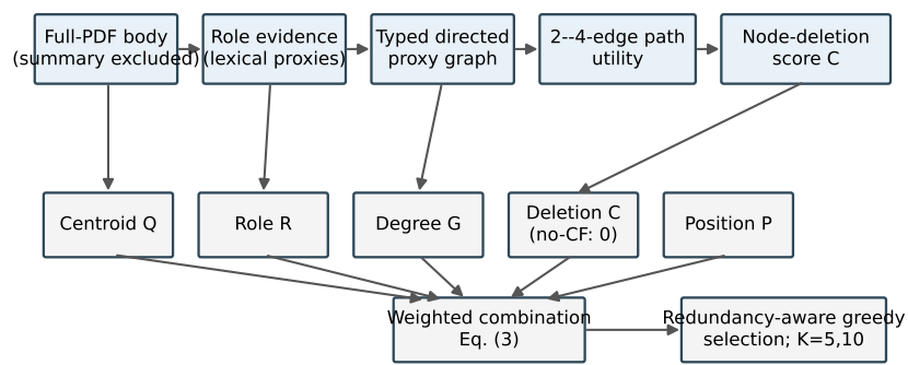
Figure 2. Implemented C^2 GES pipeline. The five channels Q, R, G, C, P enter the weighted combination in parallel; strict no-CF sets only C to zero before the same selector. Roles, edges, and node deletions are deterministic textual proxies, not a learned graph neural network, physical simulator, or causal identification.
