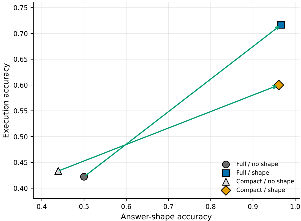
Execution versus answer-shape trade-off
