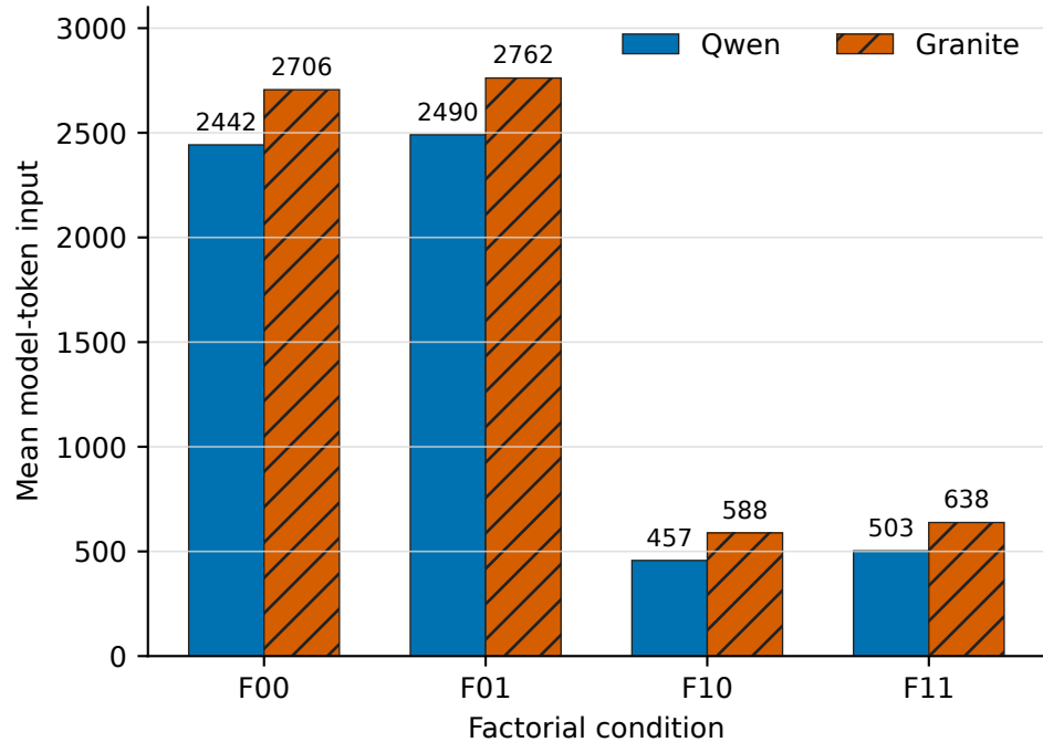
(b) Prompt-length manipulation
