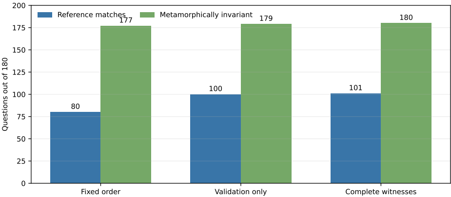
Figure 5. Descriptive release-v3 selector endpoints over 180 historical-pool questions. Reference matches are loaded only after board sealing; invariance denotes agreement across the three constructed witnesses. Bars are not a prospective multi-agent comparison.
