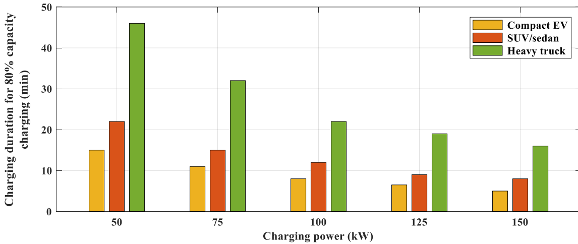
Fig. 7. Charging duration of EVs with respect to the charging power of the DC fast charger.
