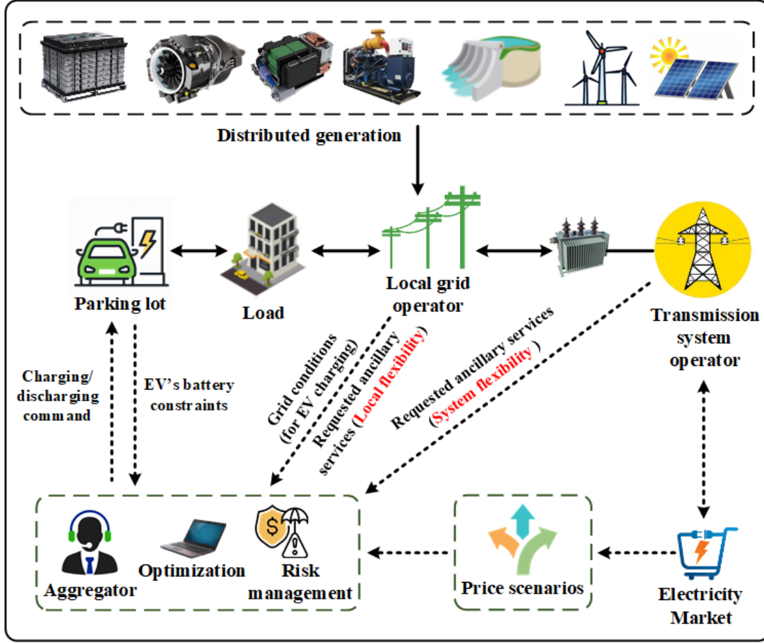
Fig. 1. Schematic diagram for electric vehicles smart charging in power systems.
