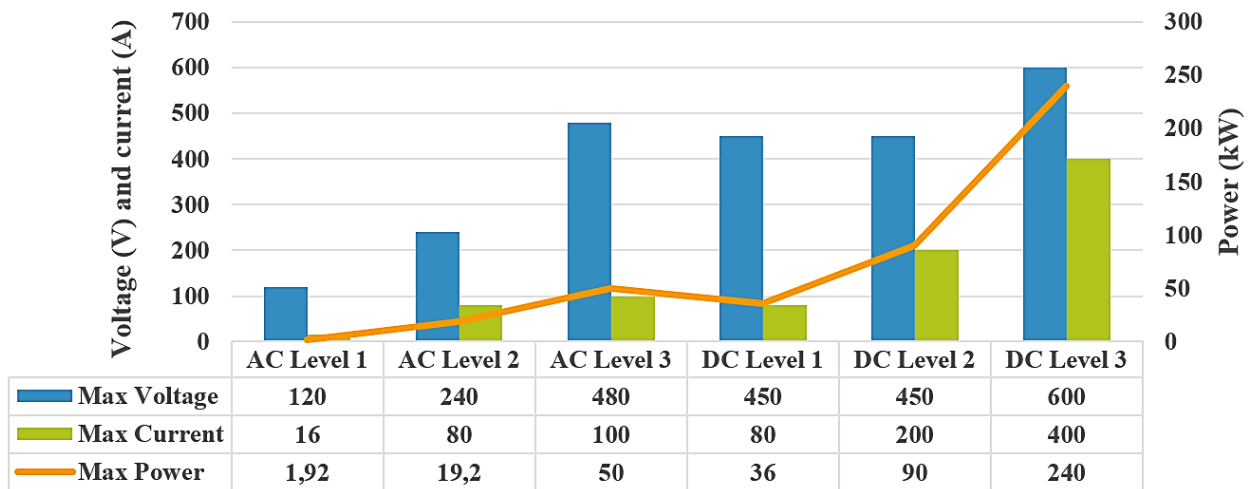
Fig. 12. Comparison of different charging levels from the viewpoints of voltage, current, and power.
