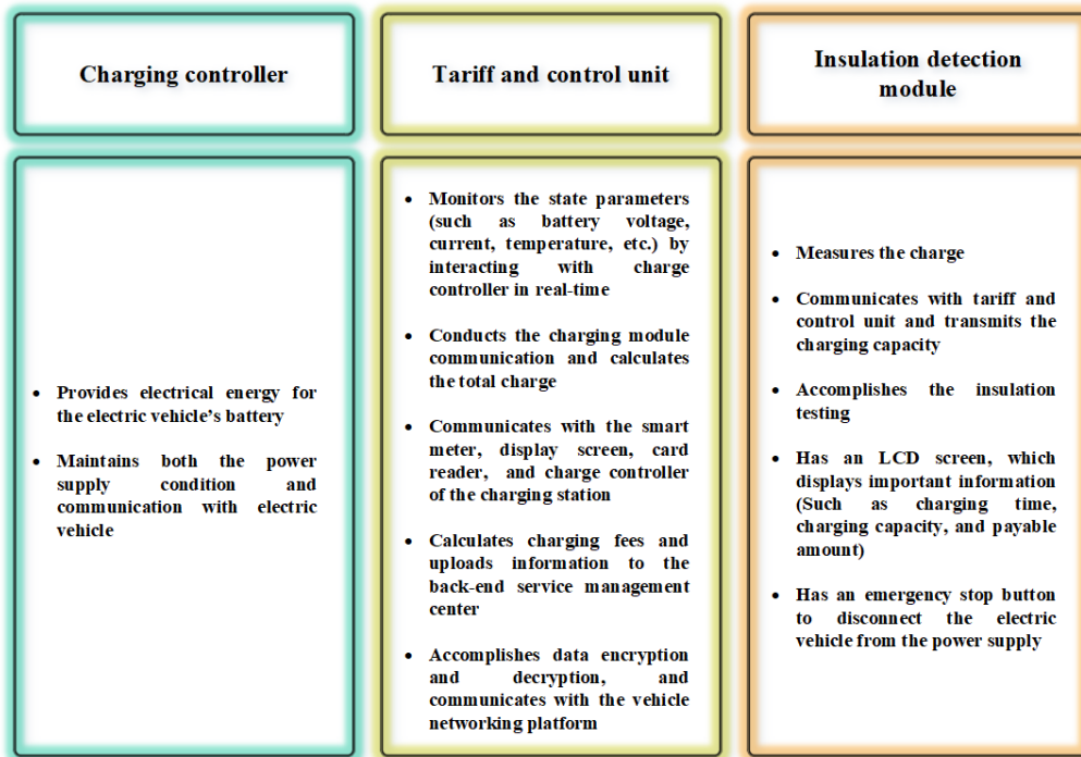
Fig. 14. Core components of DC charging systems.
