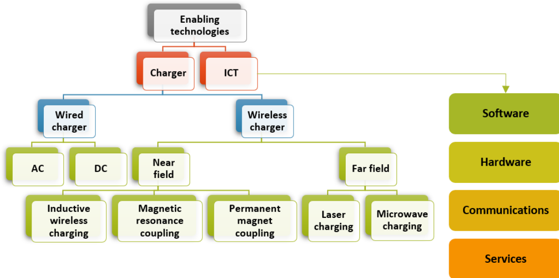
Fig. 15. Infrastructure (enabling technologies) required for implementing electric vehicles smart charging.
