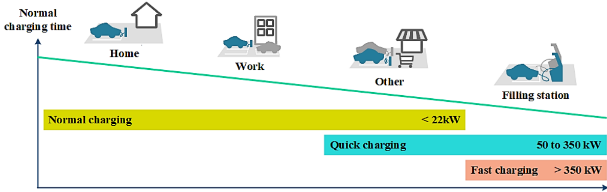
Fig. 13. Schematic diagram for charging power and time with related charging locations.
