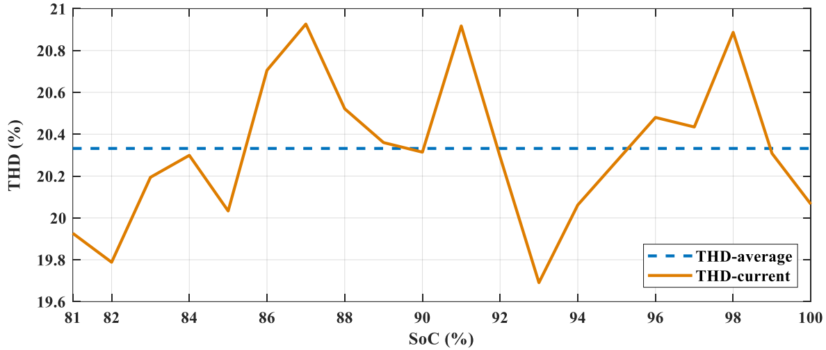
Fig. 17. Changes of harmonic distortion with respect to the SoC level for a typical problem.
