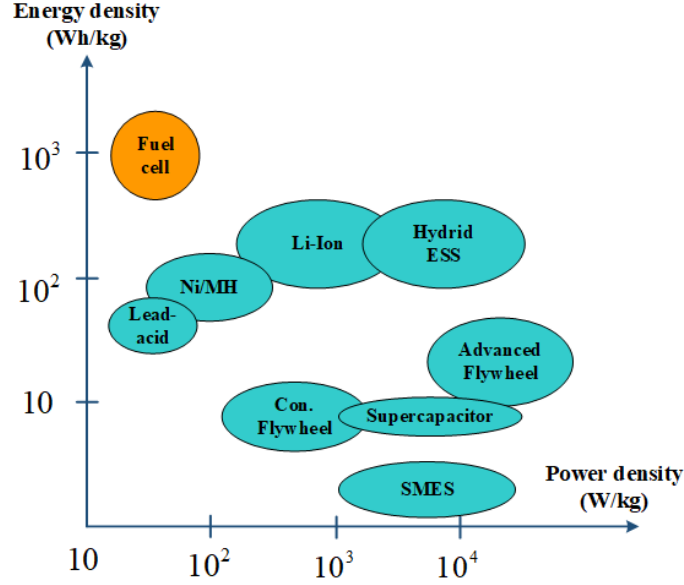
Fig. 5. Power and energy density of fuel cell compared to energy storage systems.
