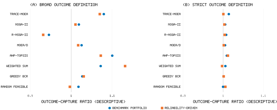
Figure 8. MTEP16 outcome-capture ratios for the two review scenarios. The dashed line denotes parity with uniform selection. Broad labels include unresolved projects among negatives; strict labels compare built projects only with explicit withdrawals. Proposed-method highlighting is visual identification and does not override the reported significance tests.
