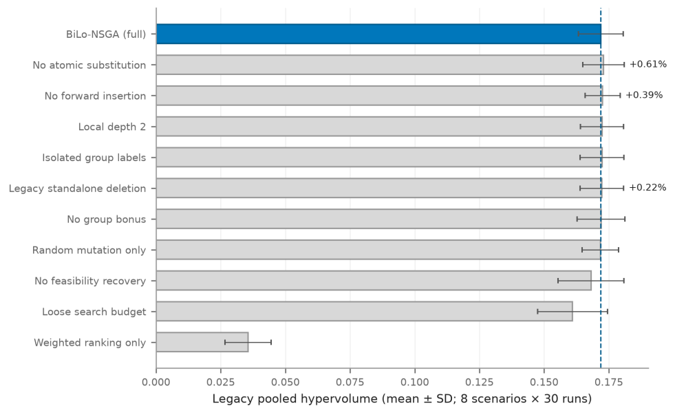
Figure 4. Mean hypervolume ( \pm std) of BiLo-NSGA and ten ablations or stress controls, pooled over all experiments and seeds. Formal decisions remain scenario-specific and Holm-adjusted.
