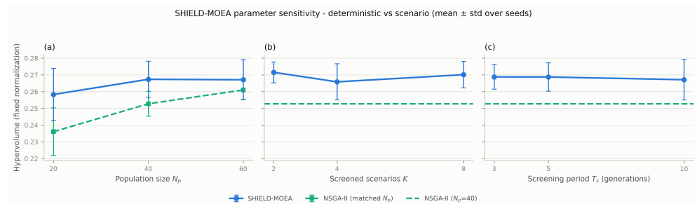
Figure 5. Parameter sensitivity over population size, screening width K , and screening period T_s (10 seeds per point; NSGA-II re-run at matched population sizes).
