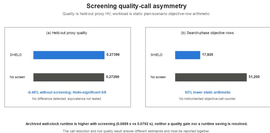
Figure 7. Screening quality–call asymmetry. (a) Pooled held-out proxy hypervolume is 0.27396 for SHIELD-MOEA and 0.27266 without screening; the within-label contrast is unresolved in 8/8 labels and equivalence was not tested. (b) The declared search code path evaluates 17,920 static plan–scenario objective rows with screening and 51,200 without it. The implementation lacks an instrumented objective-call counter, and archived wall-clock time is higher with screening, so neither a quality gain nor a runtime saving is claimed.
