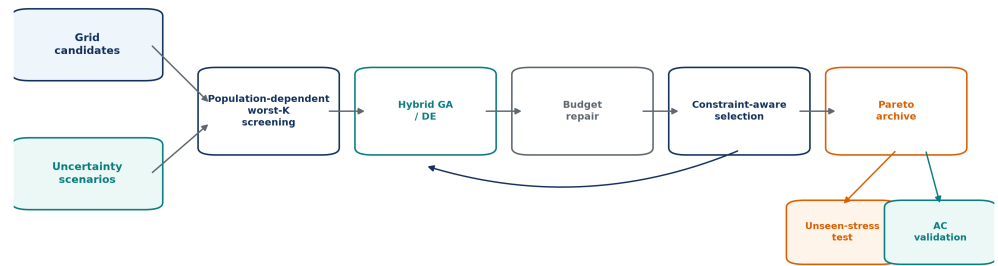
Figure 1. SHIELD-MOEA architecture. Scenario screening is population dependent; the feedback arrow denotes generational updating. The two evaluation branches use held-out stress scenarios or an illustrative AC mapping check and do not feed into selection.
