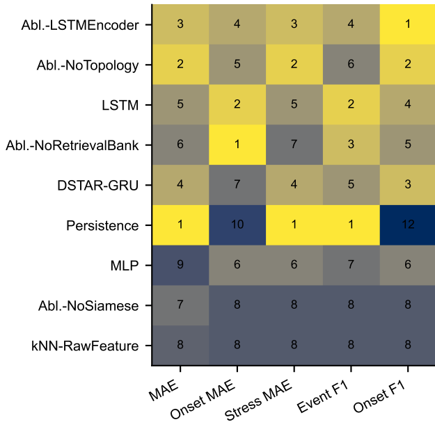
(a) 1 h: within-task metric ranks
