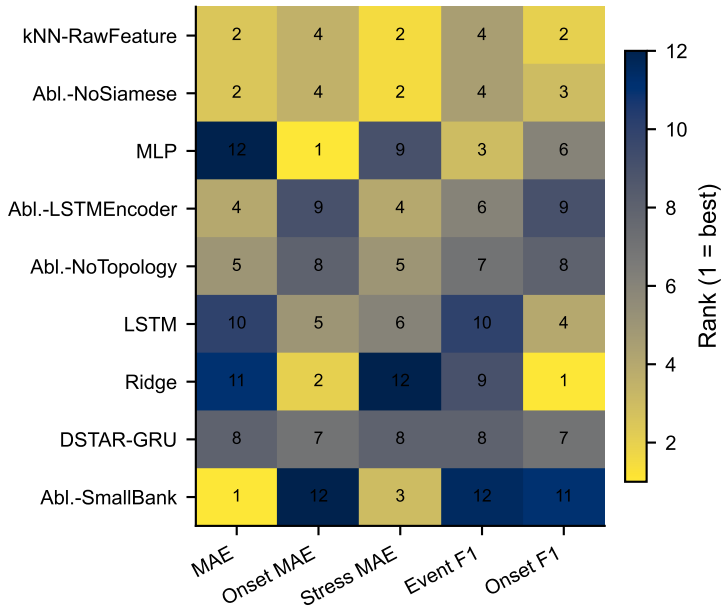
(b) 24 h: within-task metric ranks
