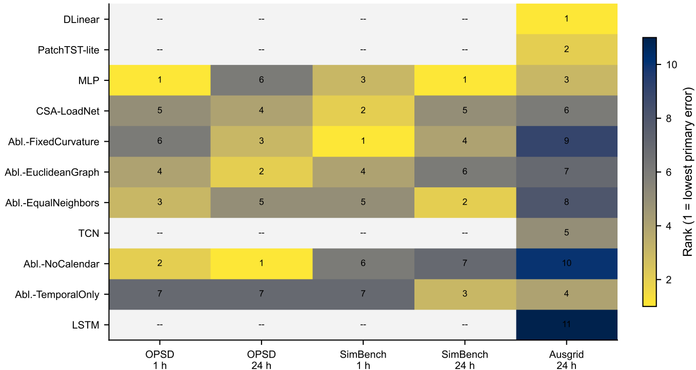
Method ranks where reported across five primary dataset--horizon settings
