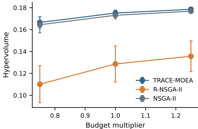
(a) Global front quality
