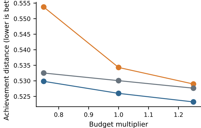
(b) Preference-region quality
