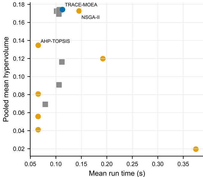
(a) Search quality and run time
