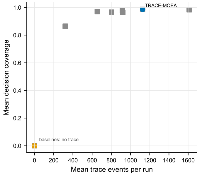
(b) Audit volume and coverage
