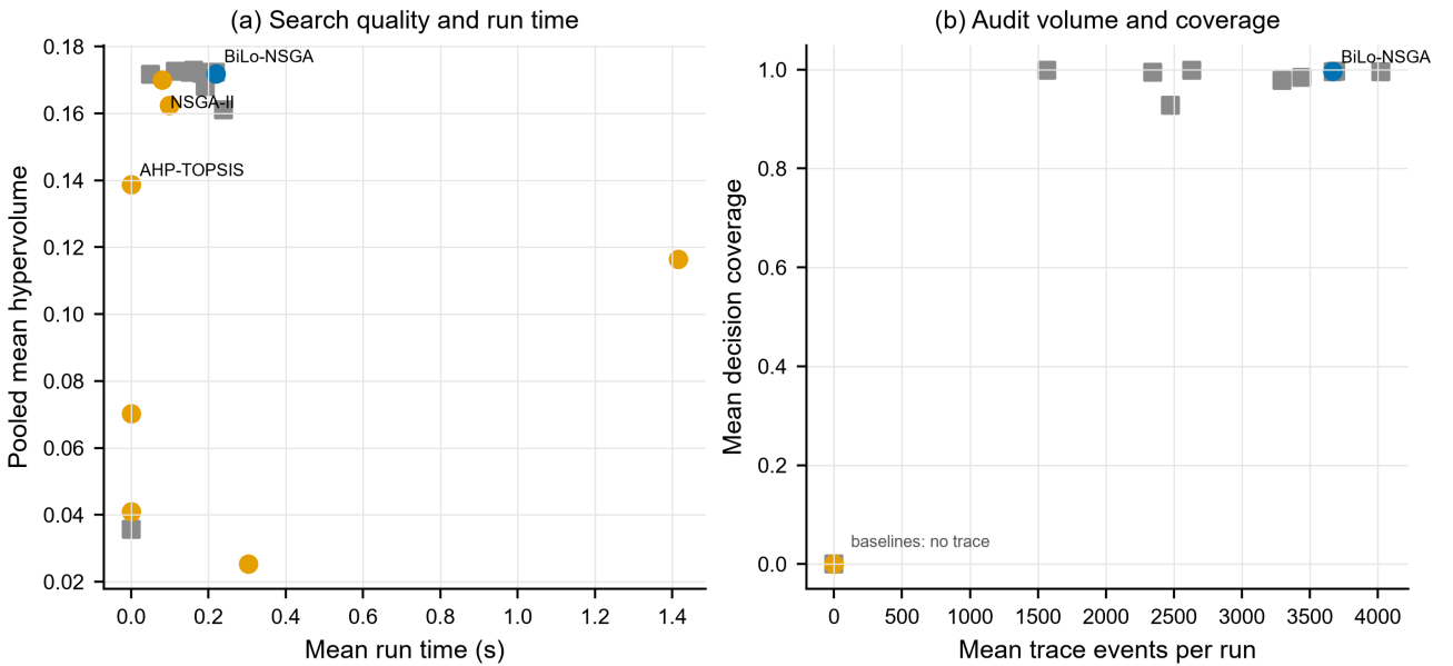
Figure 7. Pooled search-and-trace diagnostics over eight experiments and 30 seeds. Each panel retains its native unit; no composite score is formed from optimization quality and trace volume.
