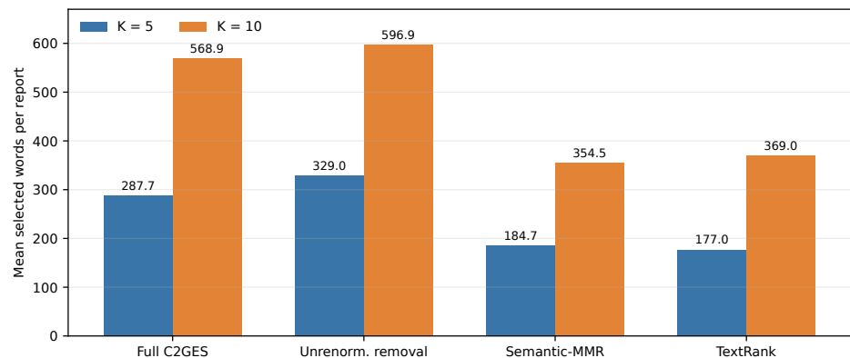
Figure 4. Mean selected words per test report for the four principal conditions. Values reproduce Table 11; no word-budget reselection was performed.
