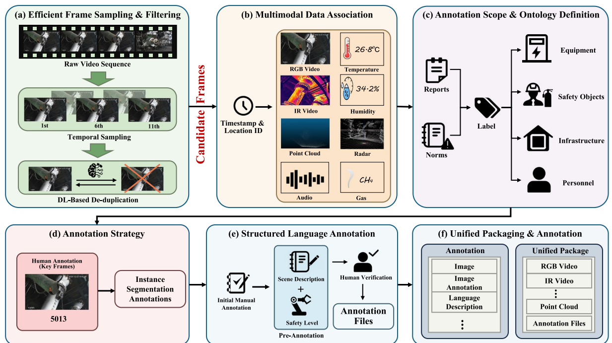
Fig. 4 Overview of the InspecSafe-V1 dataset construction pipeline.
