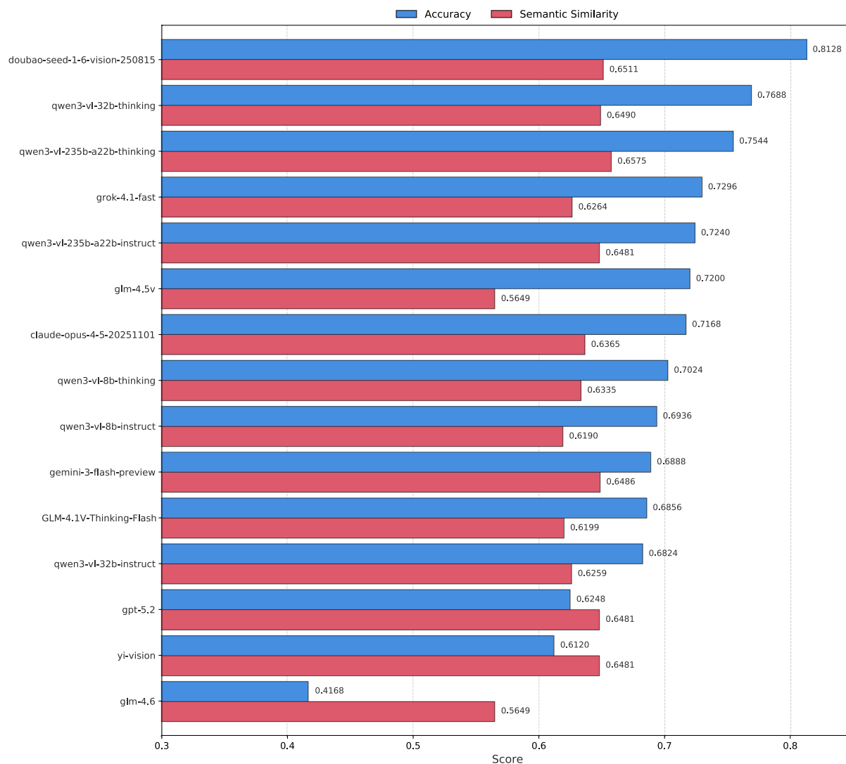
Fig. 6 Benchmark results of different VLMs on InspecSafe-V1.
