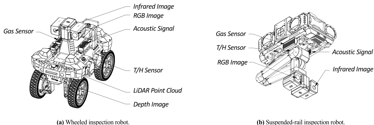
Fig. 2 Illustration of the key sensor module configurations for wheeled and rail-mounted inspection platforms.
