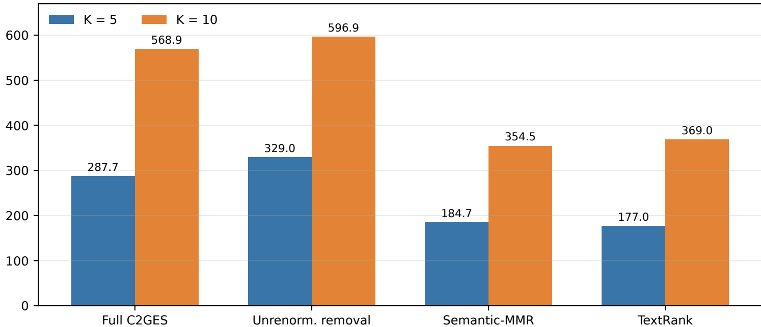
Mean selected words per report
