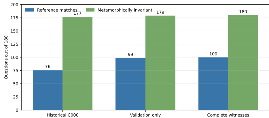
Figure 5. Selector endpoints over 180 historical-pool questions. Reference matches are loaded only after board sealing; invariance denotes agreement across the three constructed witnesses.
