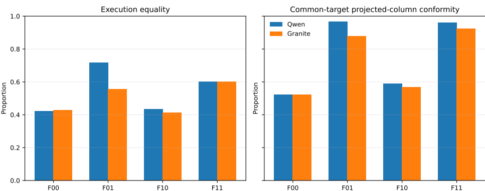
Figure 2. Audited GridDB cell point estimates. Each cell contains all 180 attempts; the figure is descriptive and does not replace the documented factorial contrasts.
