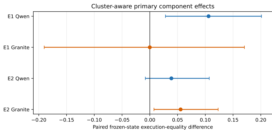
Figure 3. Component effects under a prospectively frozen call-and-selection procedure on development-visible GridDB items. Intervals describe composition sensitivity; the frozen decision rule also requires multiplicity-adjusted evidence.
