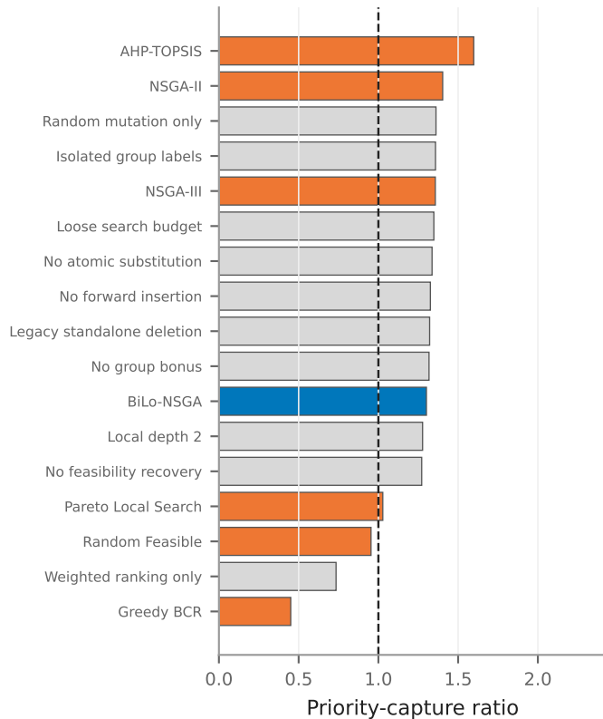
Reliability-prioritized review
