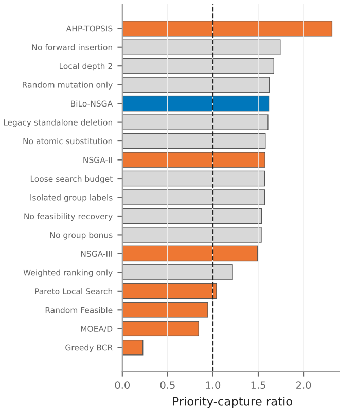
Budget-constrained selection
