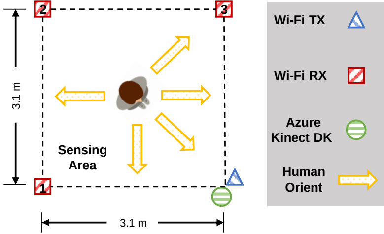
Fig. 3. Layout of Experiment Space
