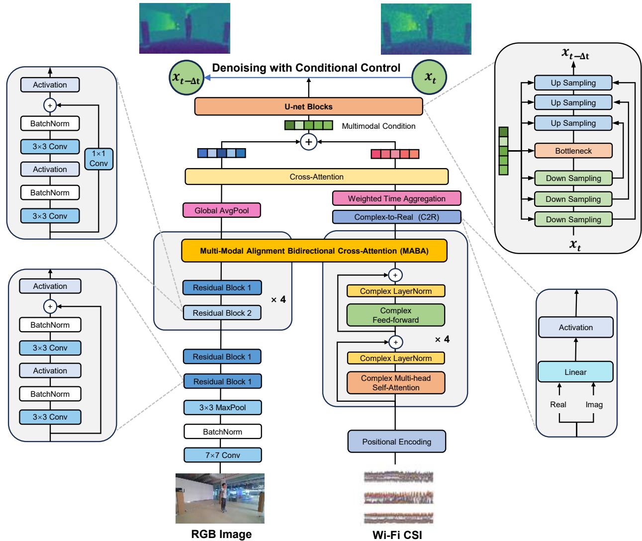
Fig. 2: Design of Denoising with Conditional Control
