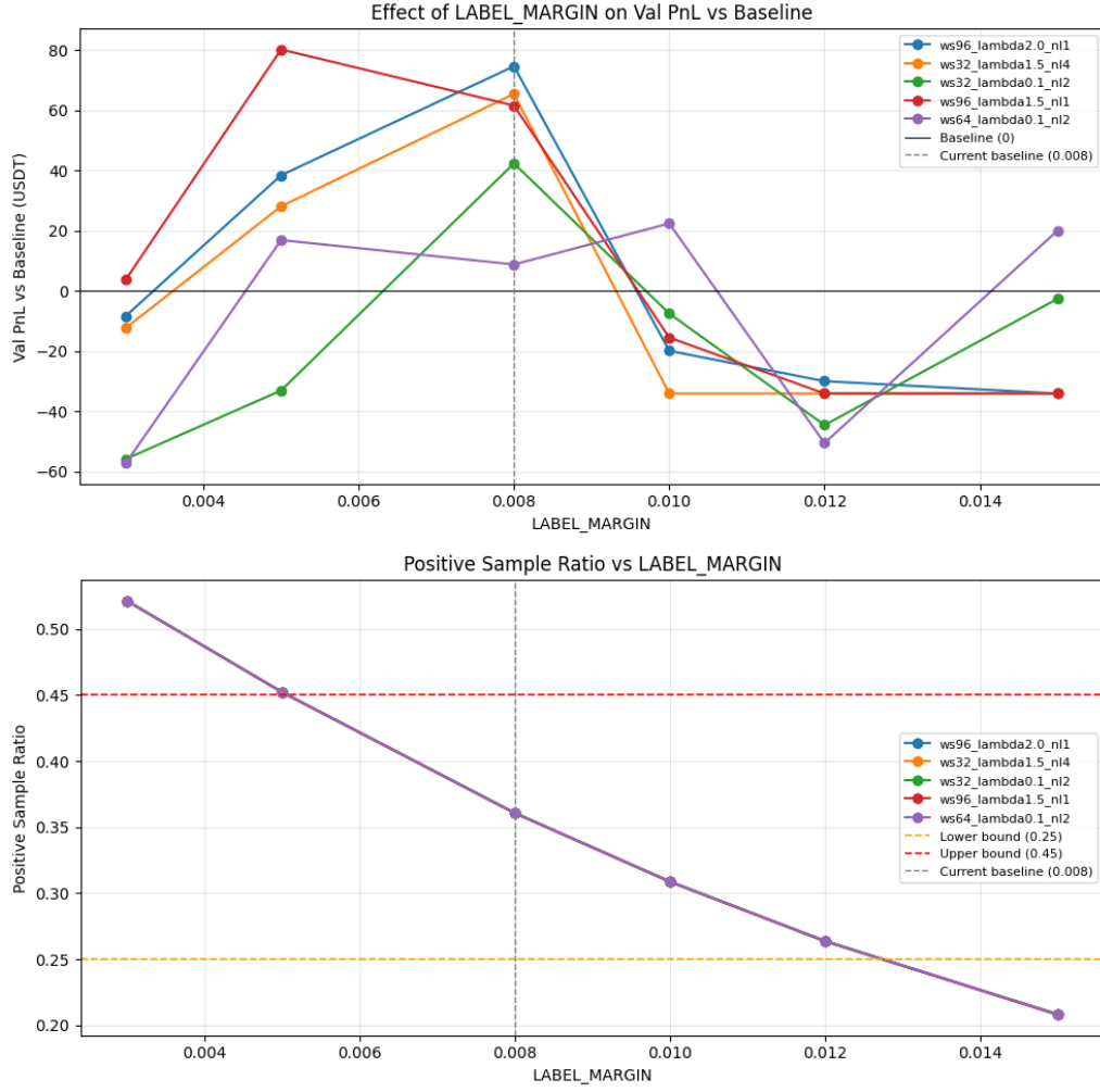
Figure B.3: Label Margin Effect - XRP
