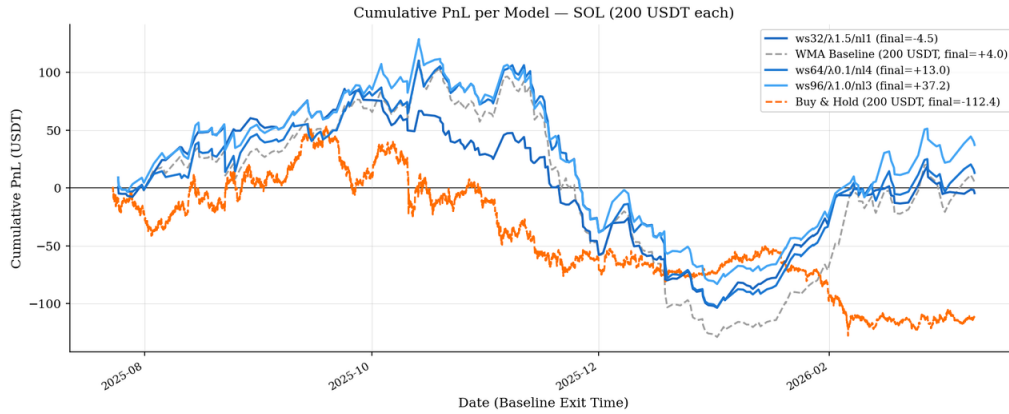
Figure B.8: Cumulative Returns of Different Strategies and Early-Closing Models for SOL
