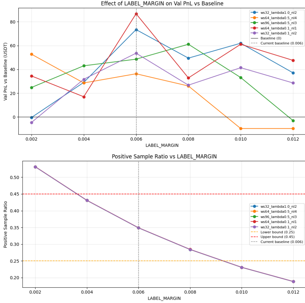
Figure B.2: Label Margin Effect - BTC
