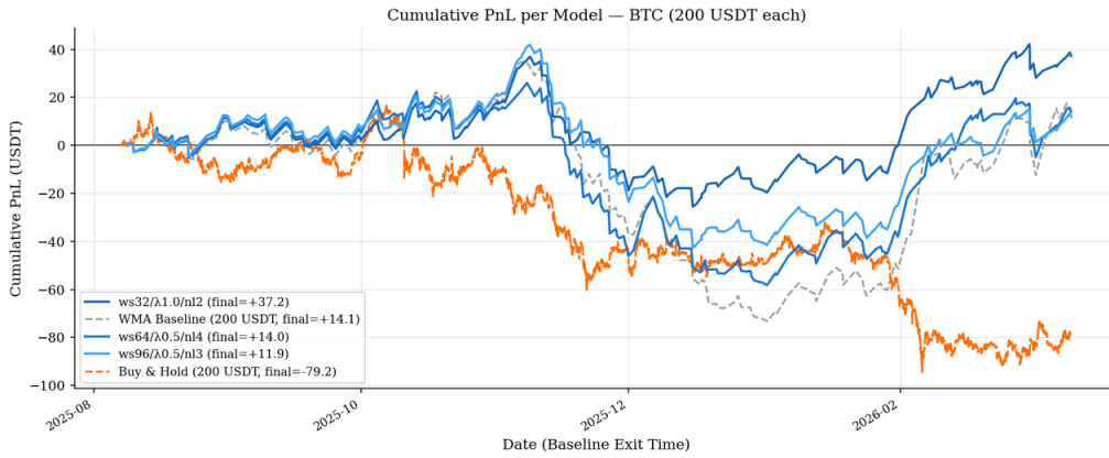
Figure B.6: Cumulative Returns of Different Strategies and Early-Closing Models for BTC
