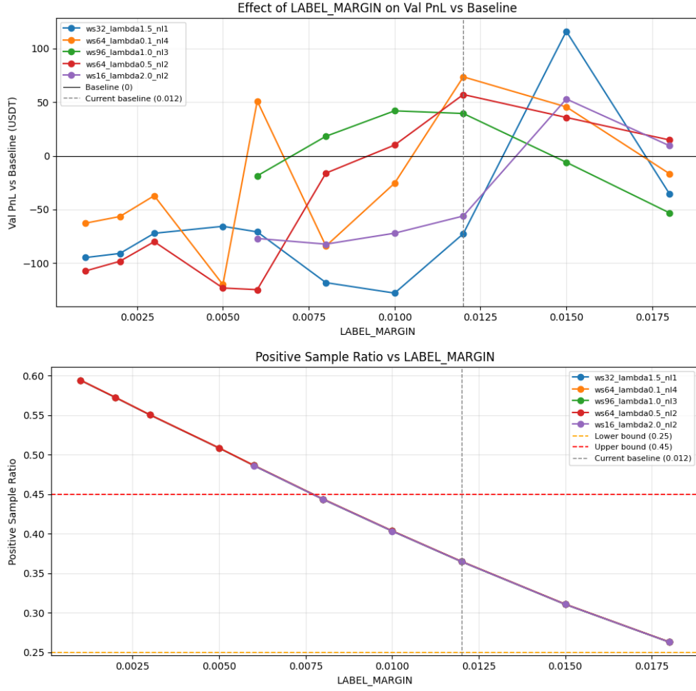
Figure B.4: Label Margin Effect - SOL
