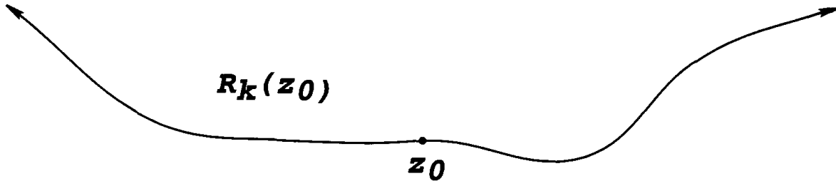
Rarefaction curve
