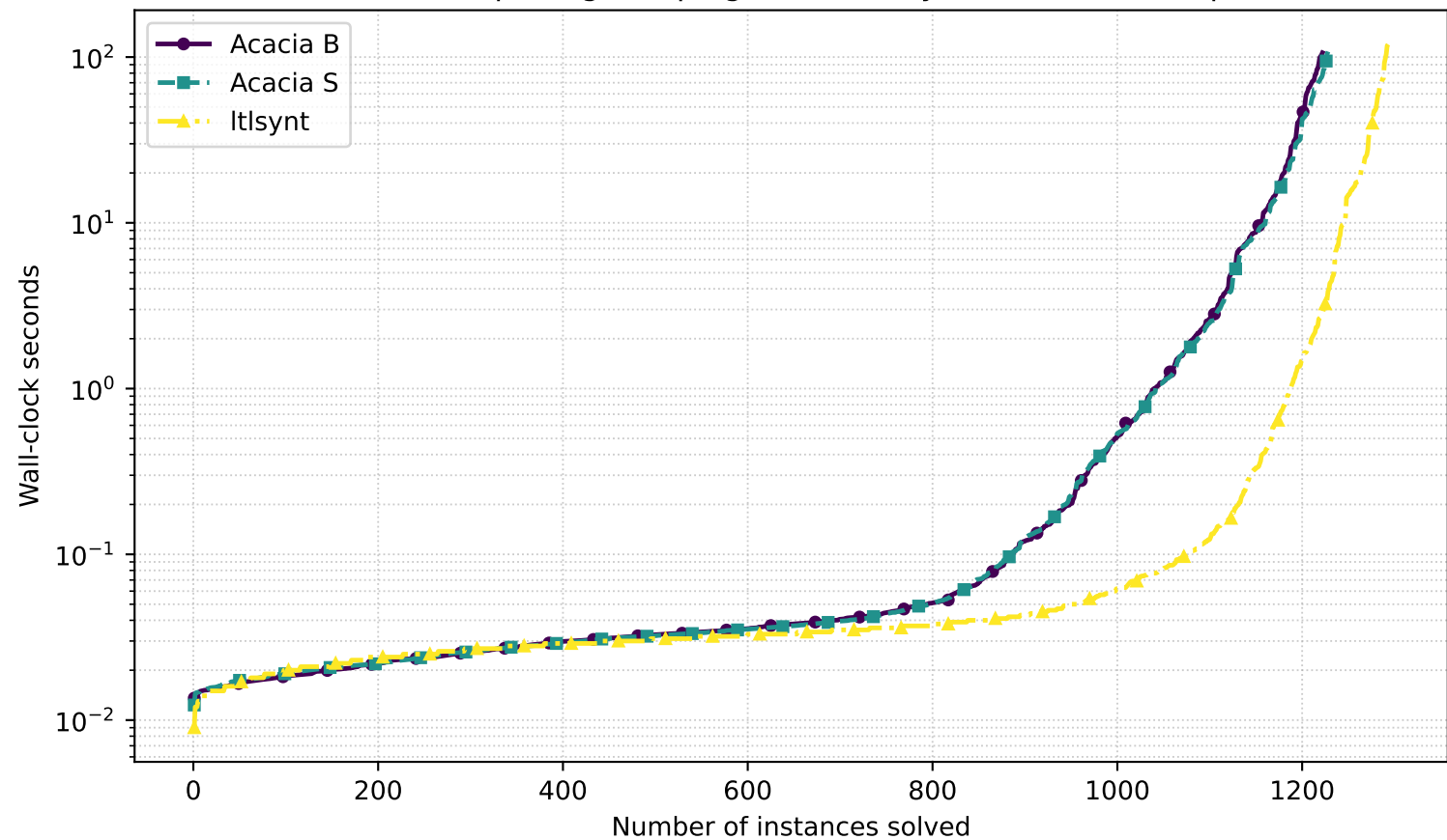
SYNTCOMP26 opening campaign — B/S/Itlsynt (120s, 8 GiB, epoch 1)
