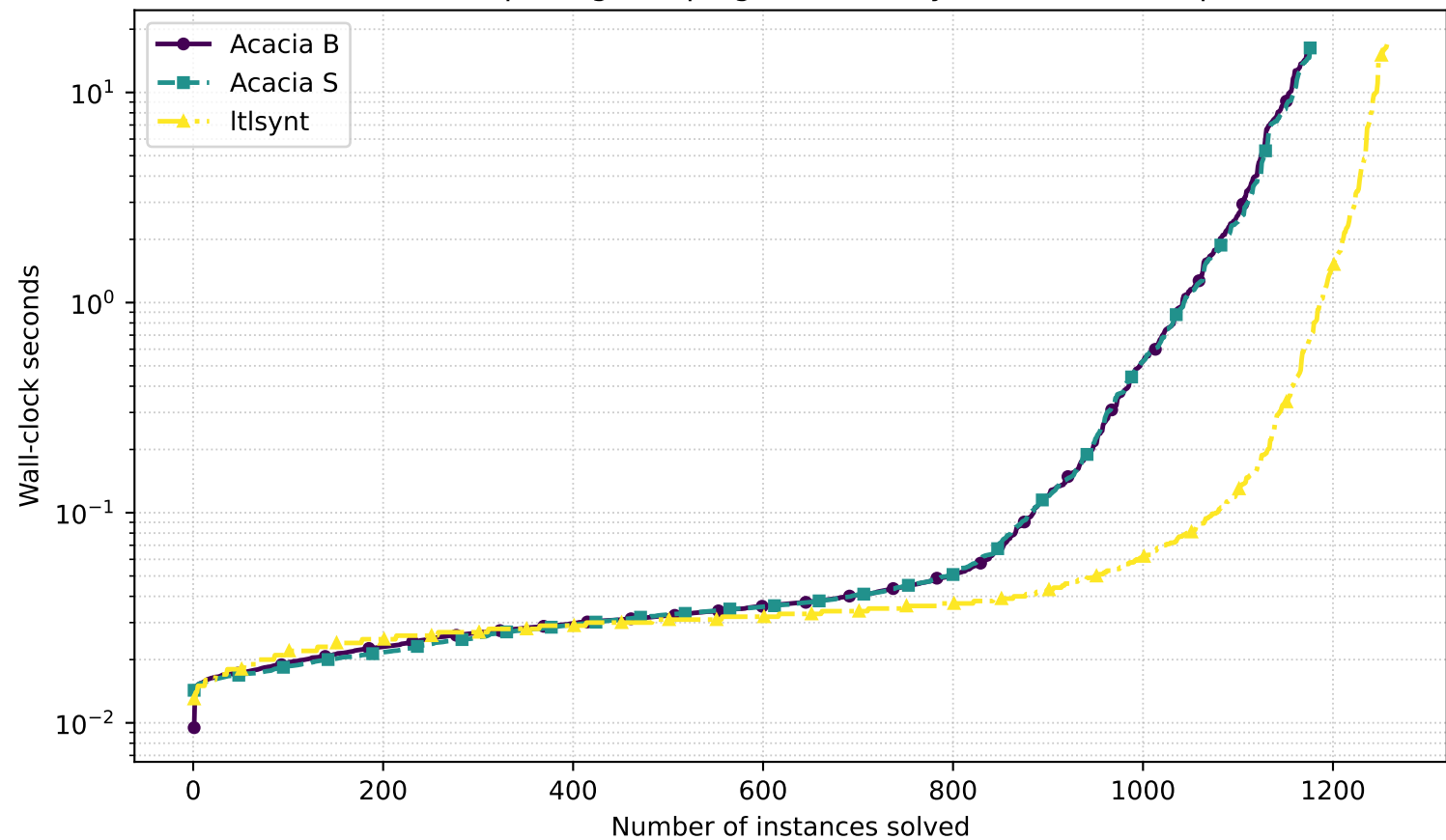
SYNTCOMP26 opening campaign — B/S/Itlsynt (17s, 8 GiB, epoch 1)
