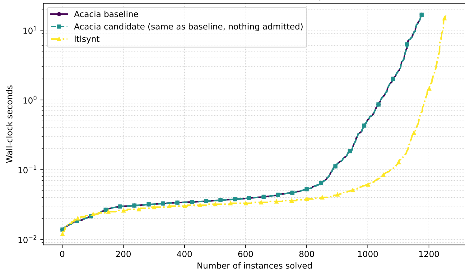
SYNTCOMP26 — baseline / candidate / Itlsynt (17 s, 8 GiB)
