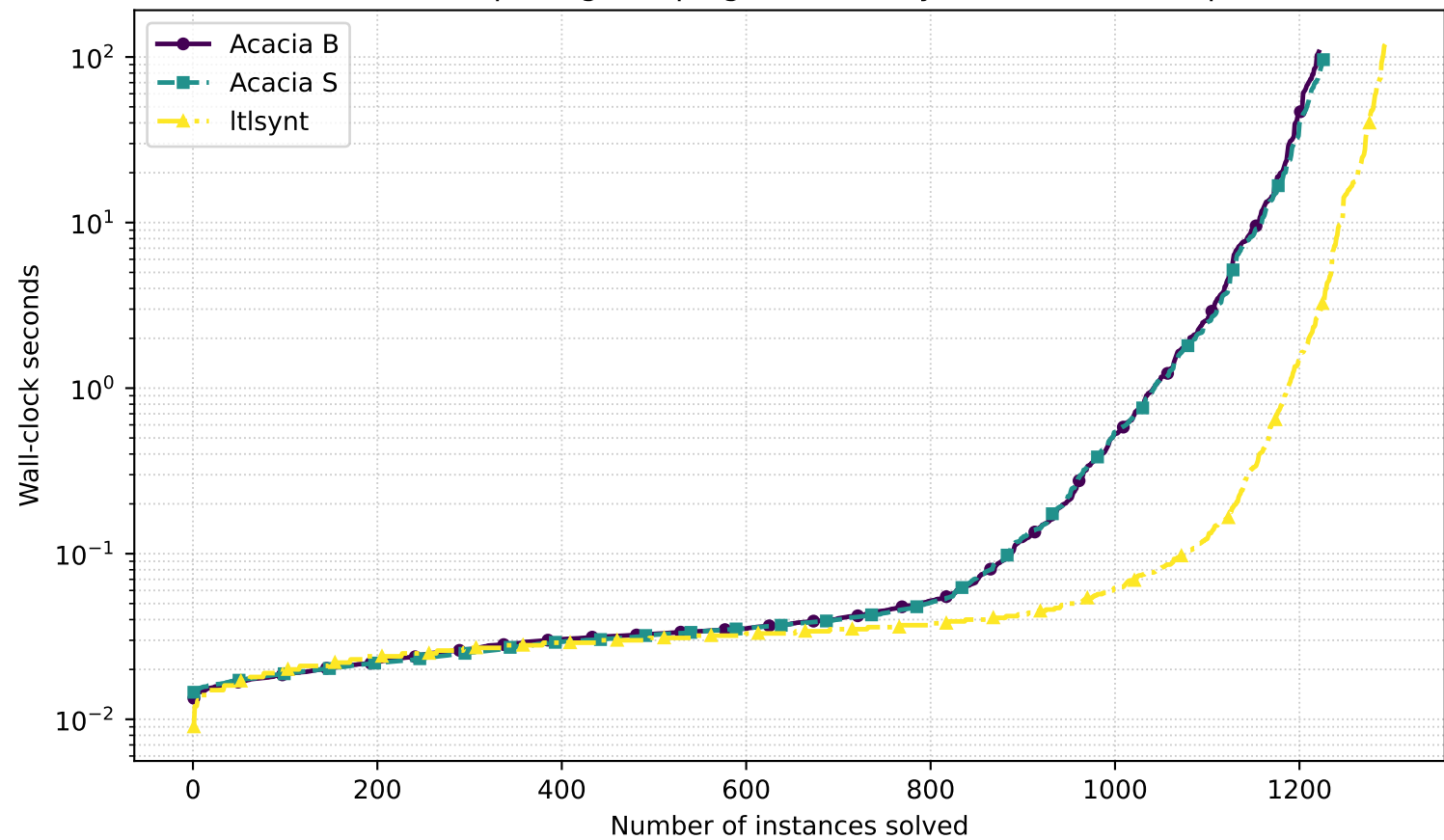
SYNTCOMP26 opening campaign — B/S/Itlsynt (120s, 8 GiB, epoch 2)
