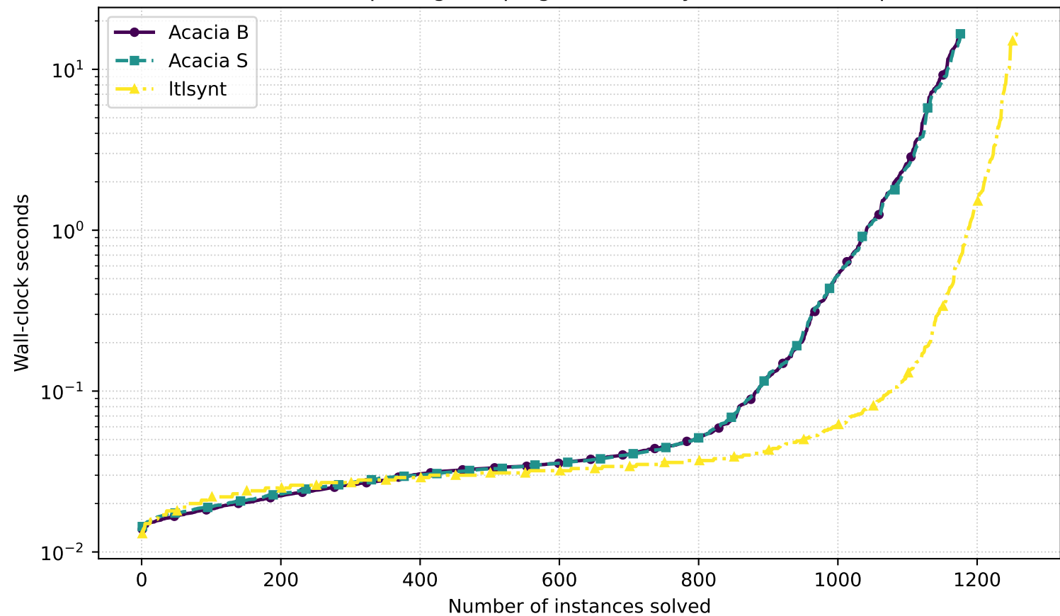
SYNTCOMP26 opening campaign — B/S/Itlsynt (17s, 8 GiB, epoch 2)
