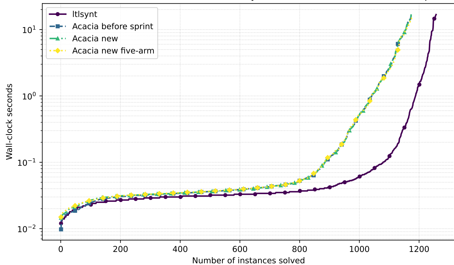
SYNTCOMP26 (1,524 instances, 17 s): Itlsynt vs Acacia before and after the sprint
