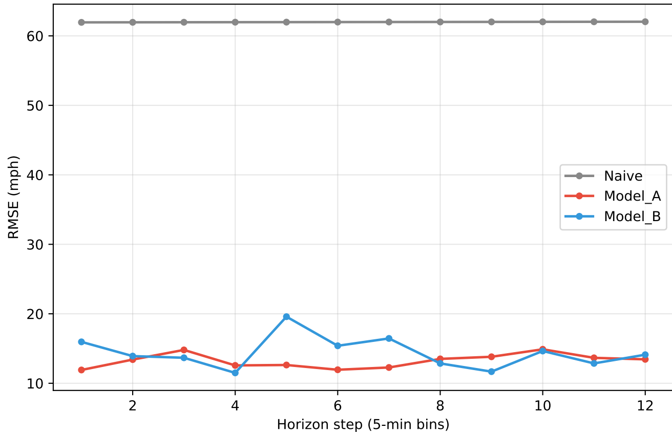
Per-Horizon Forecast Error
