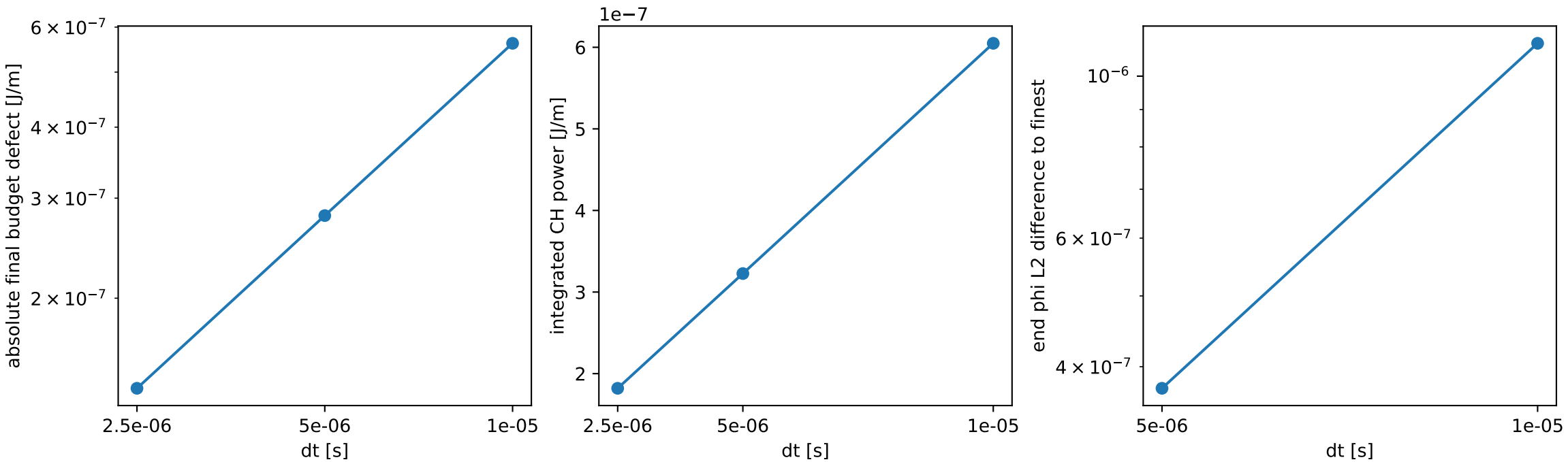
Perturbation: decreasing errors, but energy/dissipation qualification FAIL
