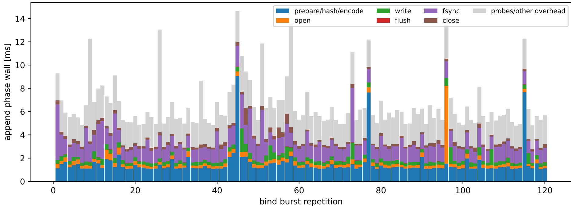
Visual zoom only: 0/120 events reach the unchanged 1000 ms stall threshold
