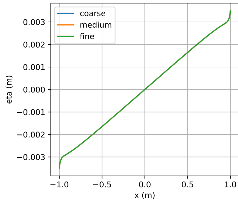
Unsmoothed P2 surface, t=0.1 s
