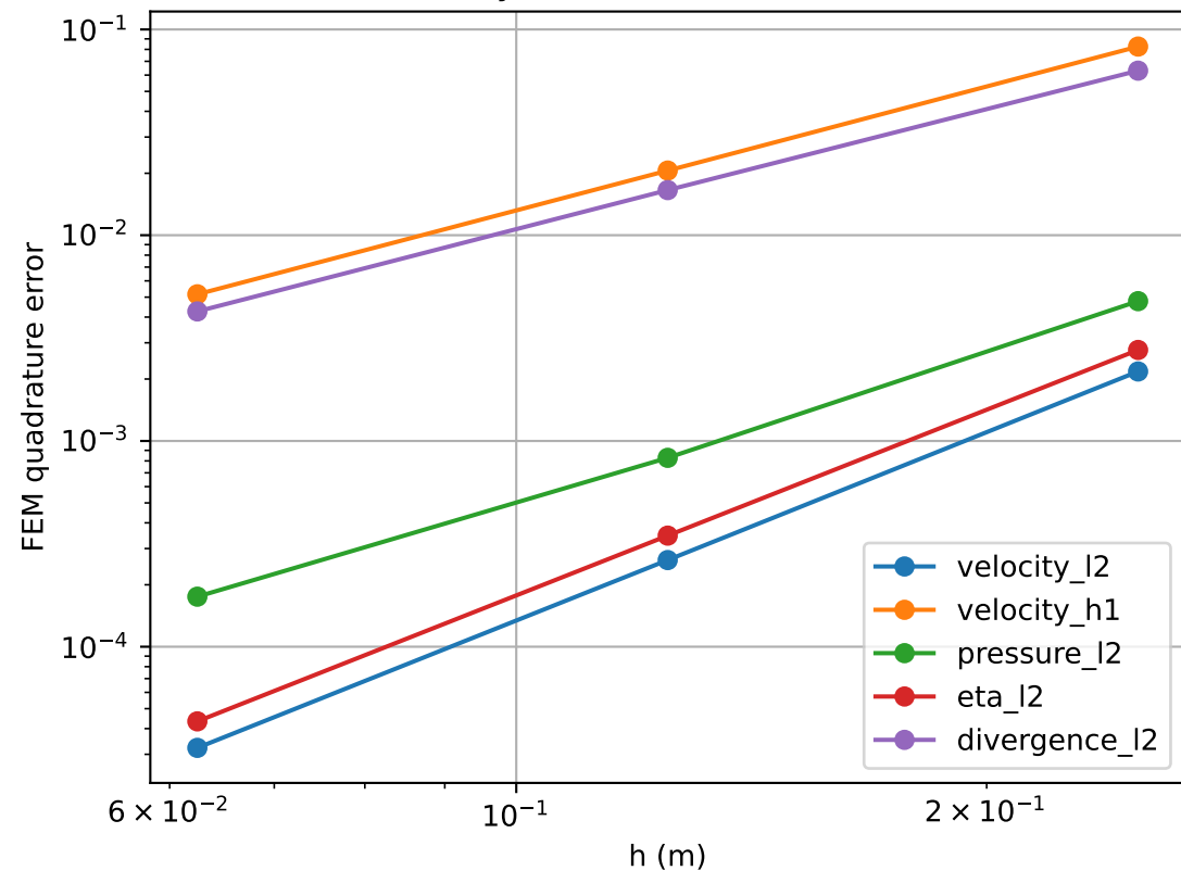
Analytic MMS, uniform mesh
