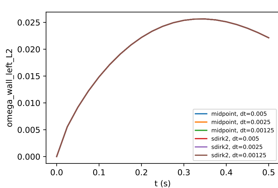
Physical temporal validation: \nu=0.01 , \alpha=0.2^\circ , medium
