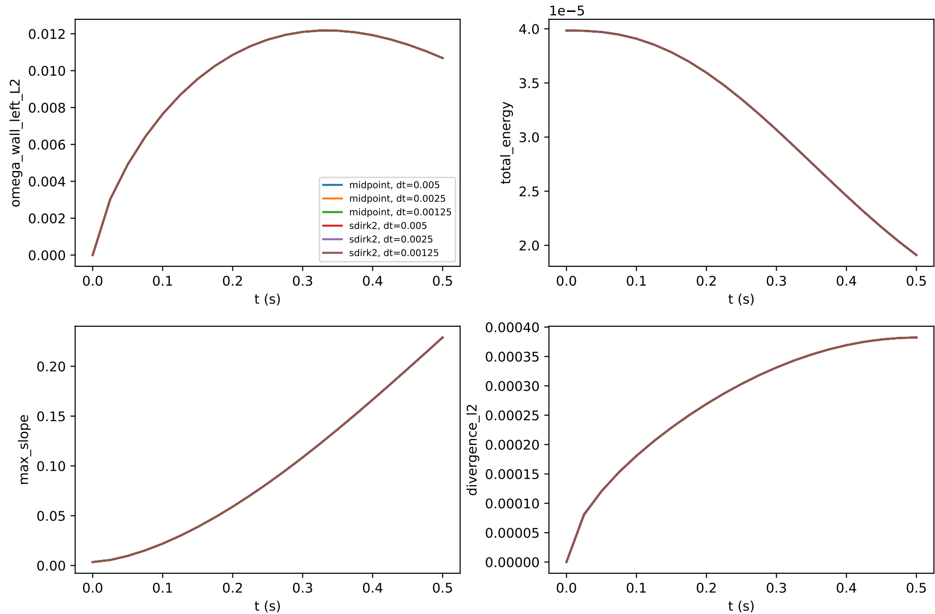
Physical temporal validation: \nu=0.1 , \alpha=0.2^\circ , medium
