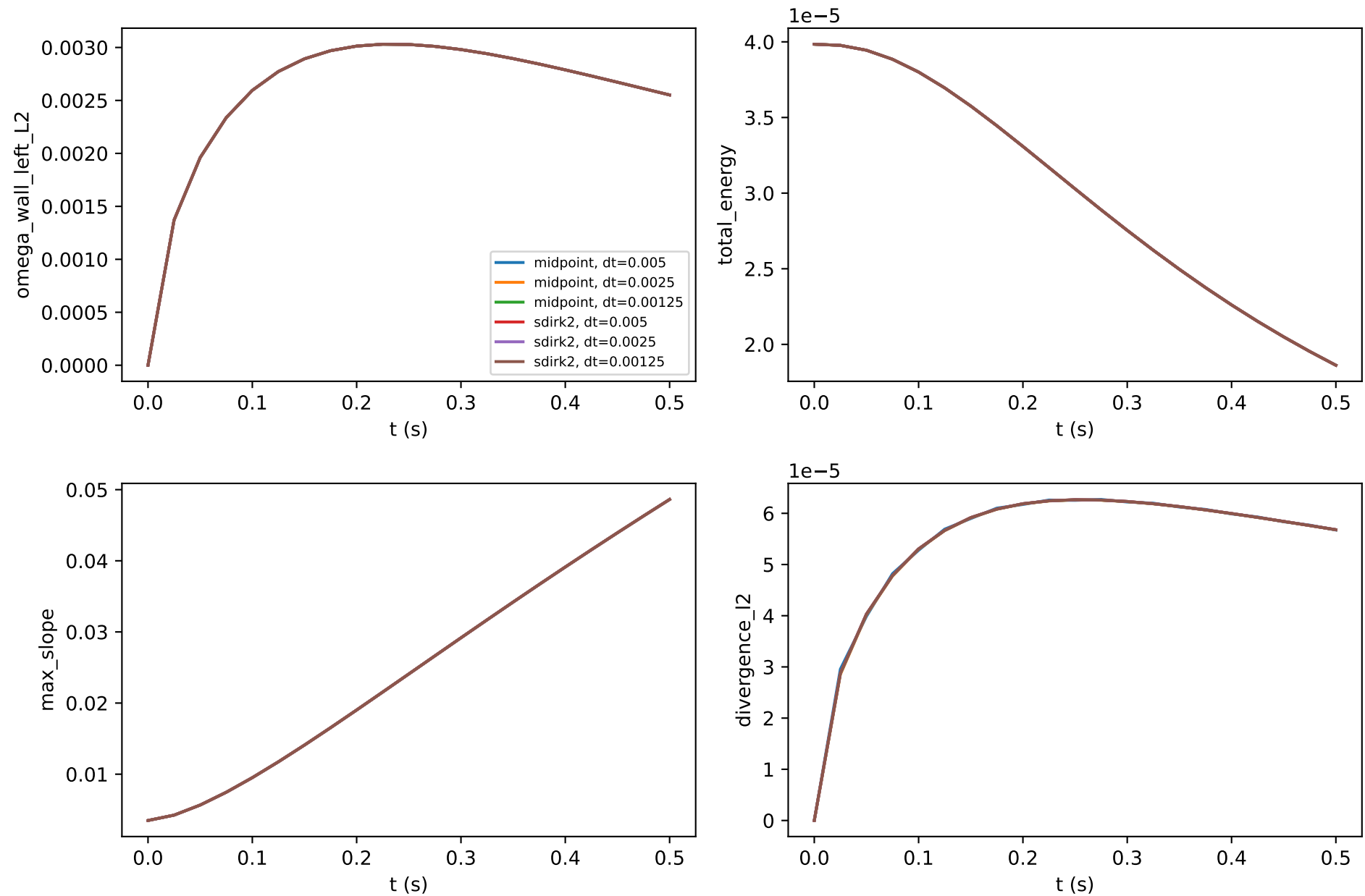
Physical temporal validation: nu=1, alpha=0.2°, medium
