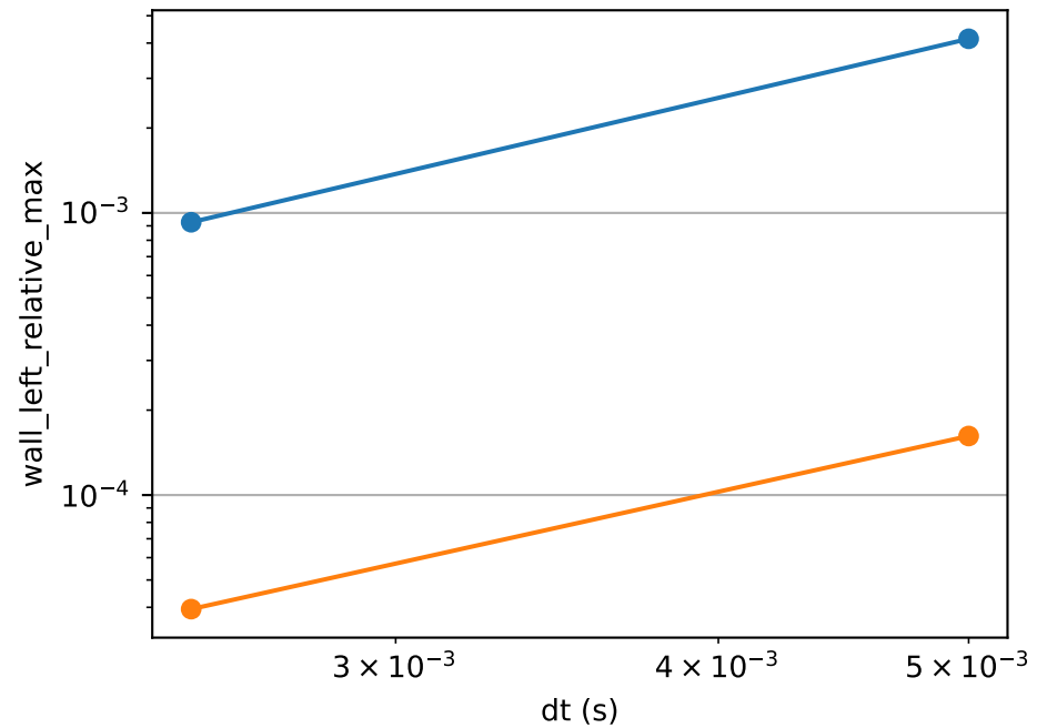
Errors versus dt/2 , \nu=0.1
