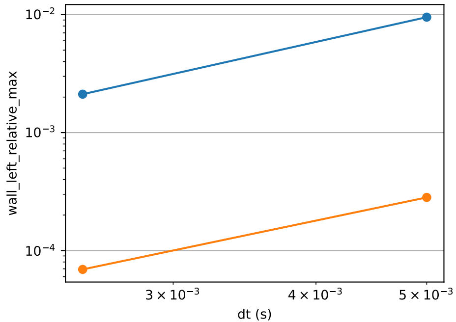
Errors versus dt/2 , \nu=1
