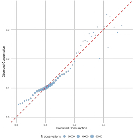
(a) Predicted vs. observed economic activity
