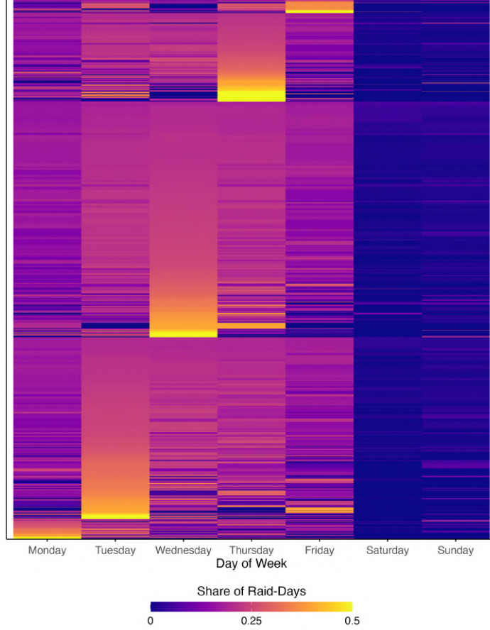
Figure 4: Heterogeneity in Weekday Enforcement Patterns Across ZCTAs
