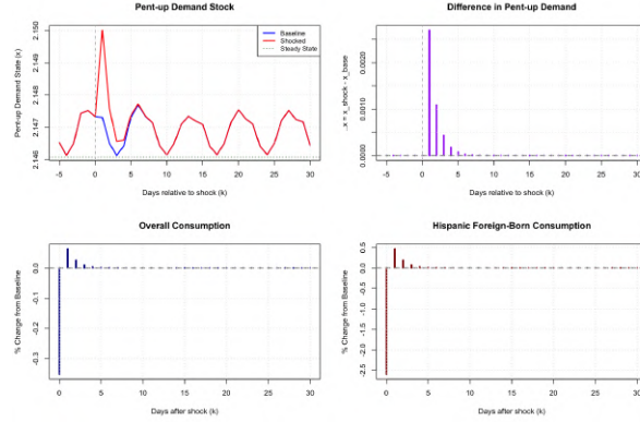
Figure A19: Impulse Response to a Belief Shock: Beliefs Evolve
