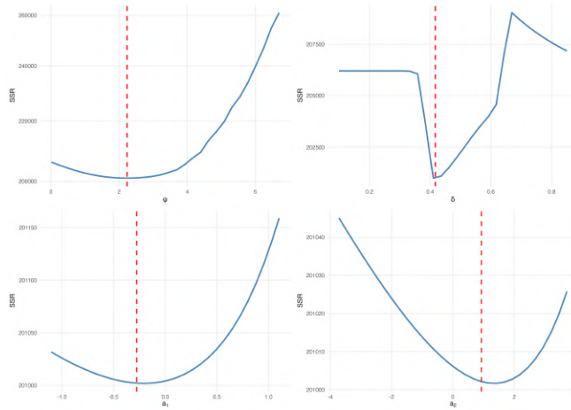
Figure A14: Profile Likelihood for Structural Parameters
