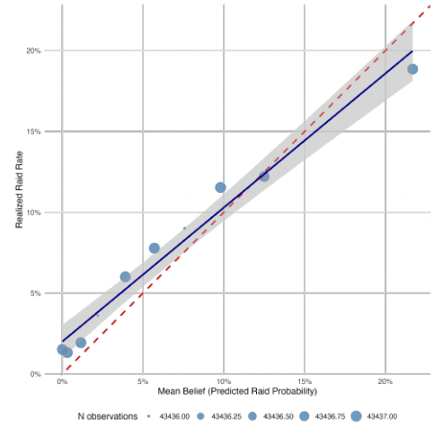
(b) Belief calibration
