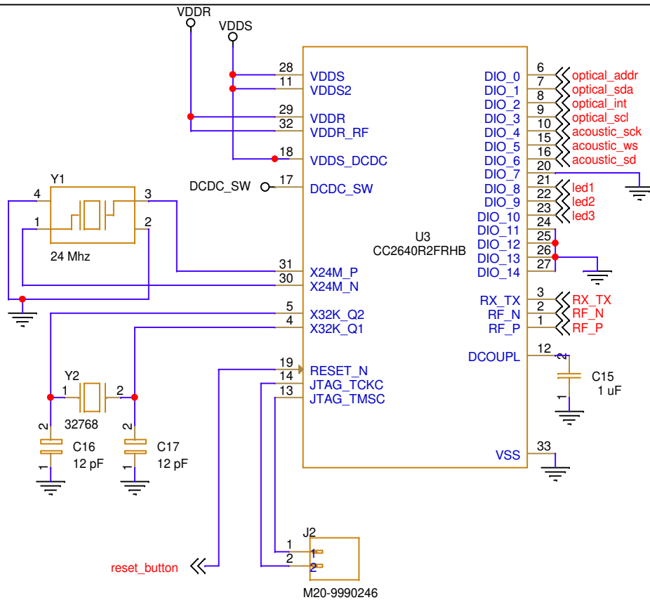
MCU circuitry
