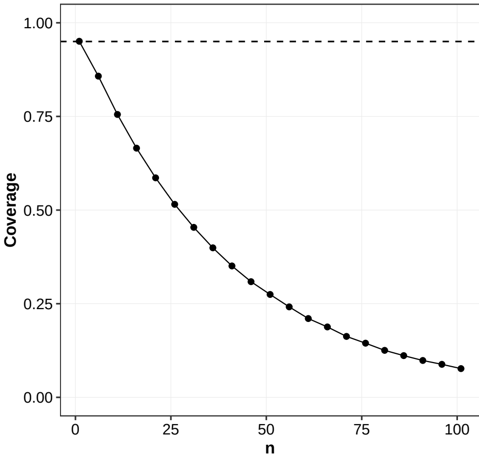
Figure 1.1: Winner's Curse Coverage
