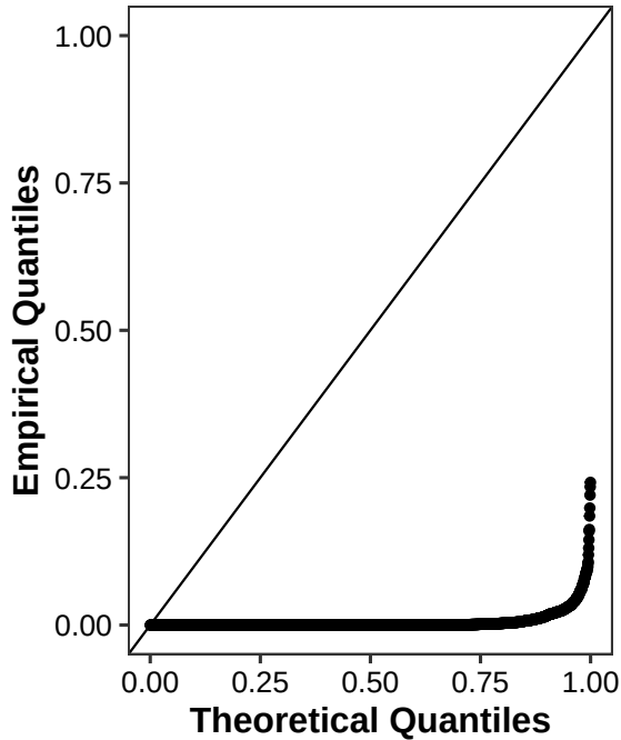
(b) Wald test
