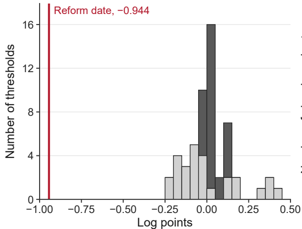
(a) Aggregate estimate, weekend \times post
