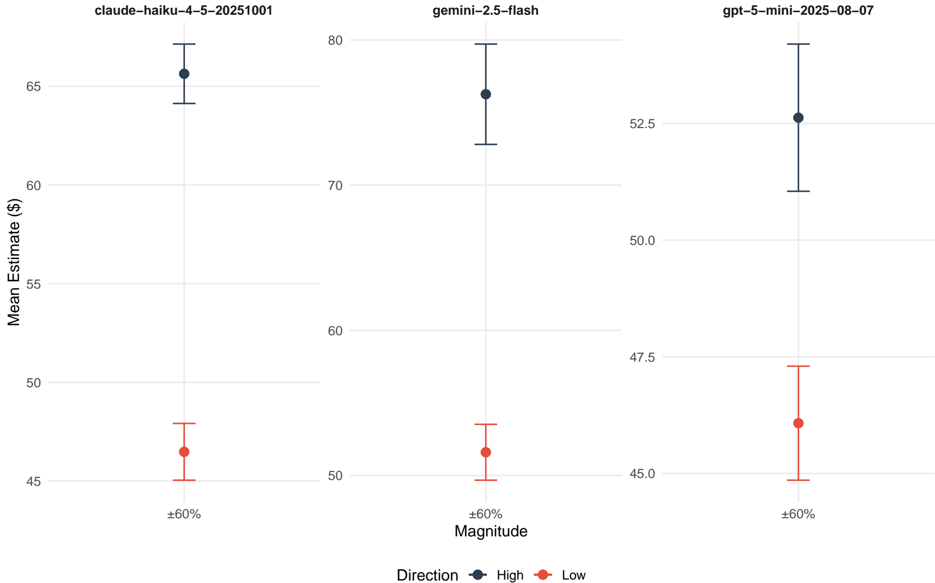
Figure 3: Anchor Magnitude Gradient (H2)
