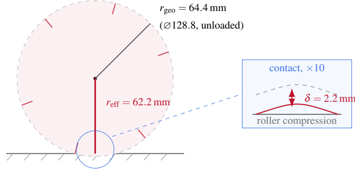
Figure 12.31: The 2.2 mm of Eq. 12.136 drawn to scale on the wheel, where it is invisible, and again at \times 10 , where it is not. That ratio is the whole reason this quantity is easy to leave wrong in a configuration file for months.
