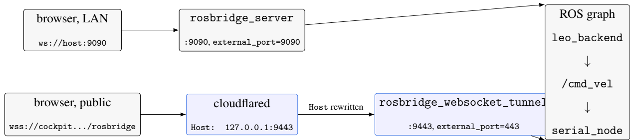
Figure 12.26: Two independent bridges reach the same ROS graph. cloudflared does not preserve the browser’s public Host header for this ingress rule; it rewrites it to the literal origin address it dials (127.0.0.1:9443), which is why the TLS bridge’s external_port is set to 443 — the public port implied when a real browser’s Host header carries no port at all — and not to 9443.
